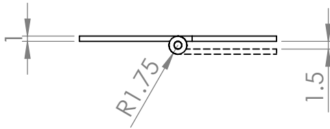
DETAIL A SCALE 1 : 1
