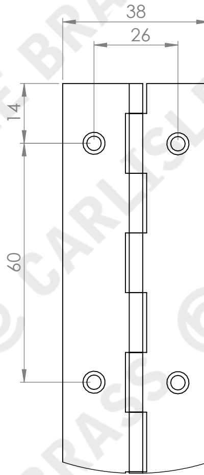
DETAIL A
